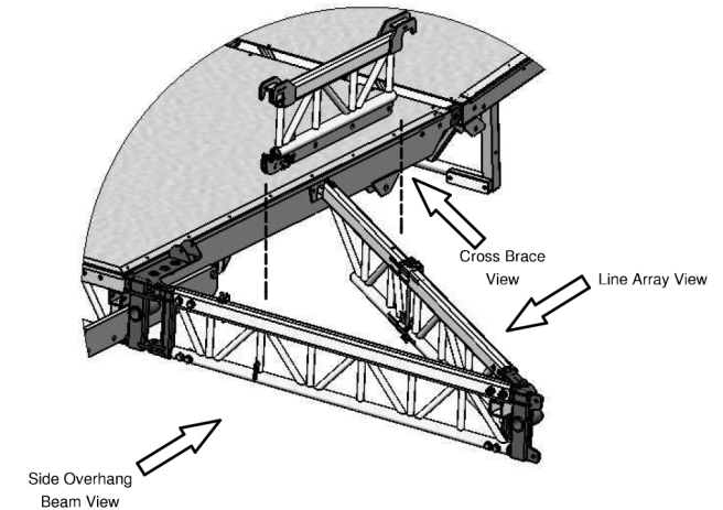
Optional Line Array Structure
